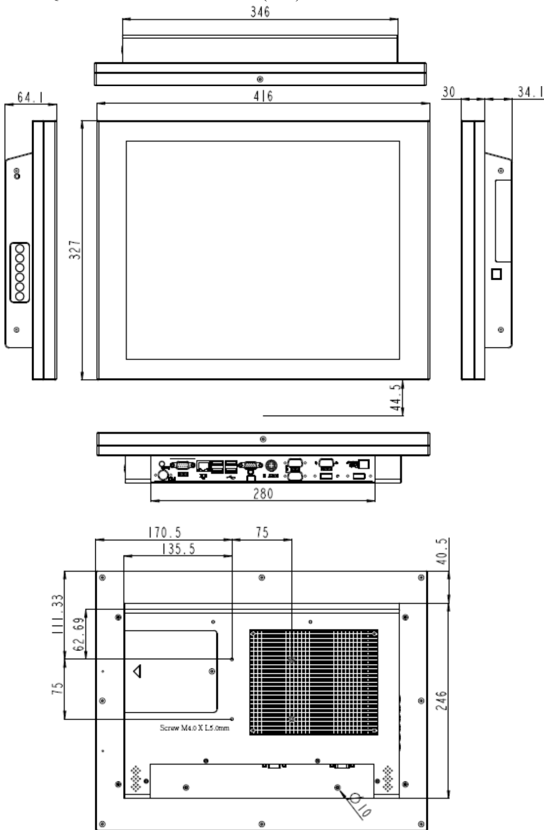
Panel PC QYT-MPPC817 Dimensions (mm)
